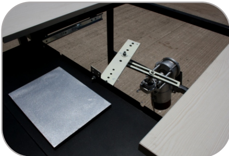
Slide Testing Machine for Quality Assurance of slides
